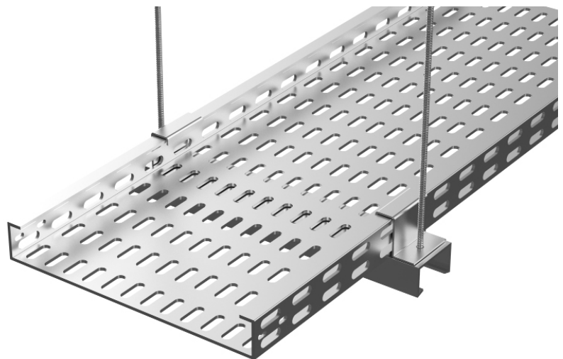
Hold Down Clamp
